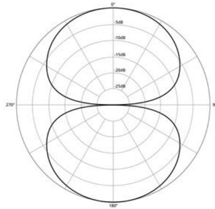
Bi-directional (Figure 8)
