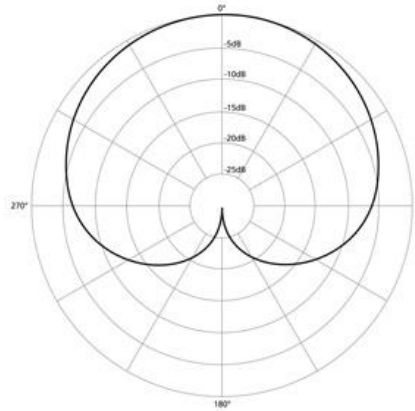
Unidirectional (Cardioid)
